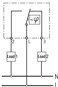
Connection Diagram
